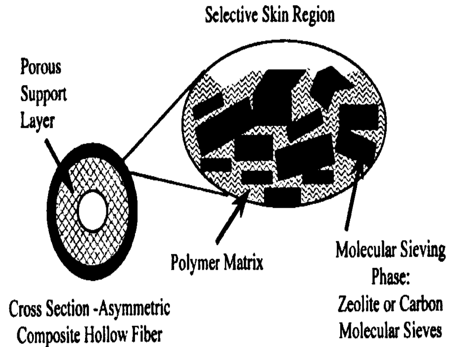
Fig. 5. Schematic of a mixed matrix membrane.
