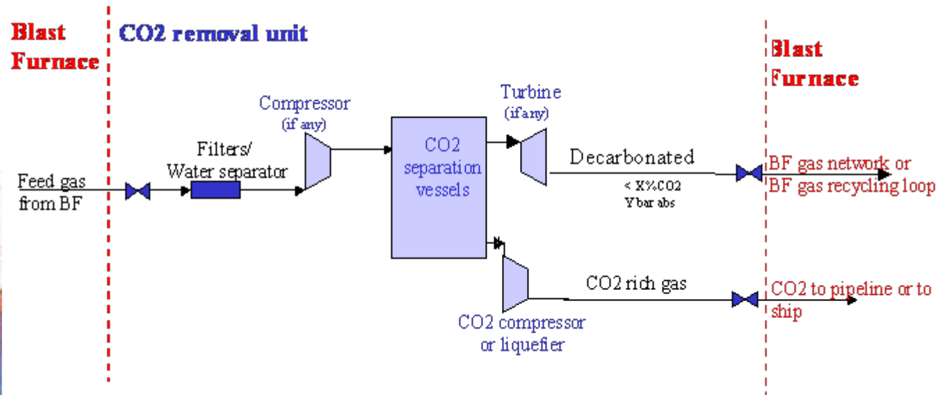
Location of the CO 2 removal unit in the steel production process
